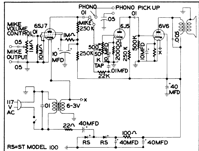
AUDIO AMPLIFIER
