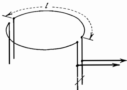
FIG. 50.—Alford receiving type ultra-high-frequency loop antenna.
