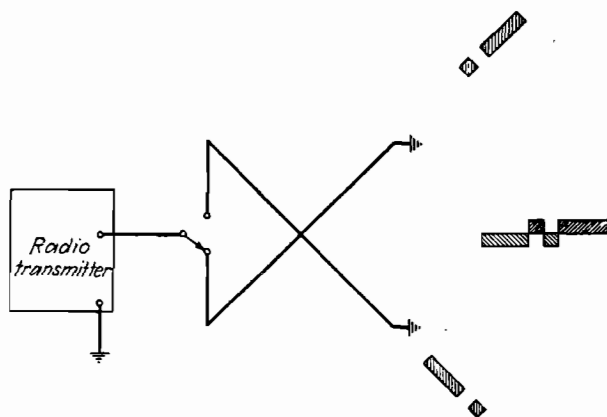
FIG. 14.—Diagrammatical representation of the principles of the aural radio range.
