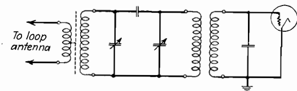
FIG. 56.—Filter circuit used to increase the image frequency rejection in an ultra-high-frequency receiver.
