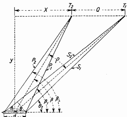
FIG. 85.—Loop taking bearings when close to a range station. The individual towers induce individual voltages in the sides of the loop.
