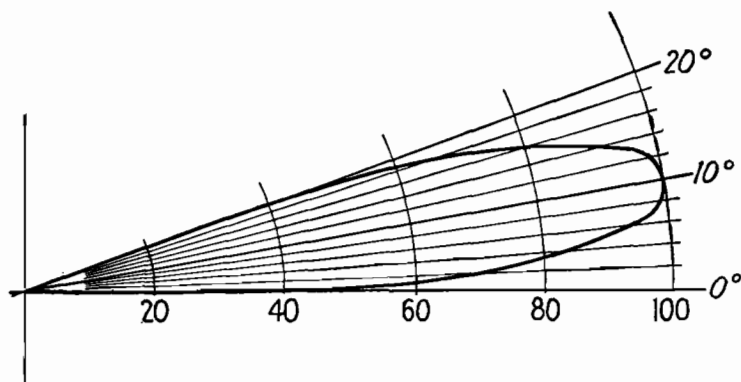
FIG. 112.—Vertical field pattern of an antenna.
