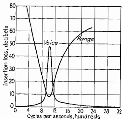
FIG. 29.—Characteristics of the filters used for simultaneous radio-range reception.
