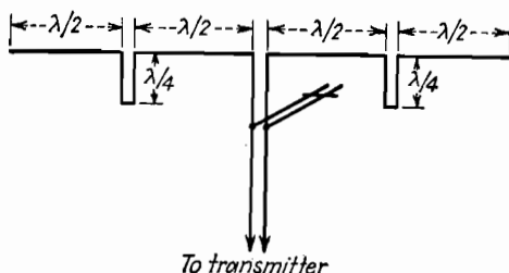
FIG. 102.—Fan-marker antenna array.
