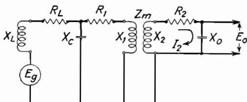
FIG. 74.—Equivalent circuit of low-impedance loop system of Fig. 73.
