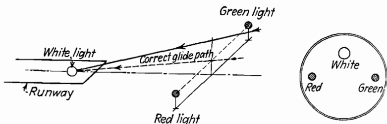
FIG. 130.—If the airplane is in line with the runway but above the correct line of descent, the center light appears as shown.
