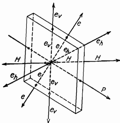
FIG. 146.—Rotation of the electric and magnetic vectors in an abnormally polarized wave.
