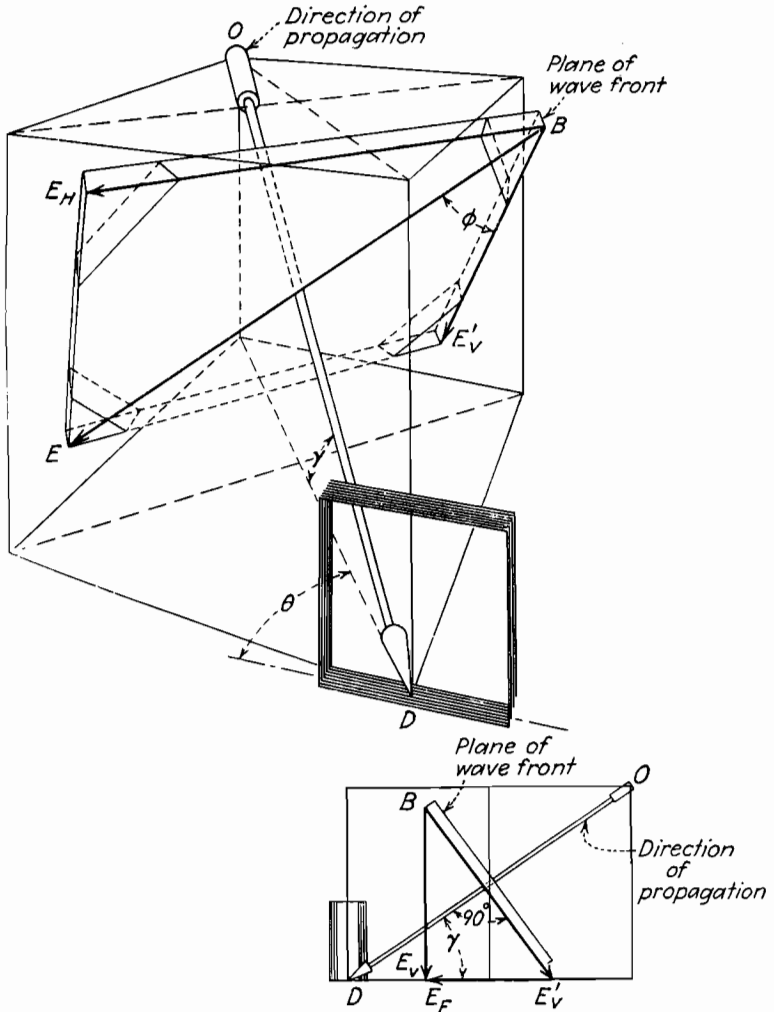
FIG. 147.—Abnormally polarized wave arriving at a direction finder from the ionosphere. The electric field, EB , is resolved into two components, E_HB and E'VB , in the plane of the wave front. The component E'VB is further resolved into two components, E_F and E_V . The component, E_F , is horizontal and in the direction of propagation. The component, E_V , is vertical.
