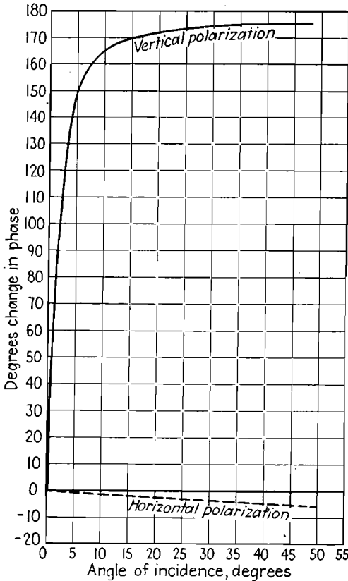
FIG. 43.—Change in phase between the incident and reflected ray for various incident angles but for soil of a given conductivity and dielectric constant.
