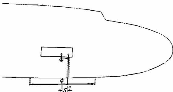
FIG. 106.—Antenna for receiving 75-megacycle marker beacon signals.
