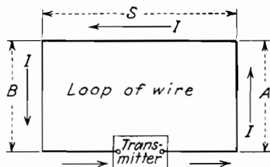
FIG. 9.—Current flowing in a simple loop antenna.
