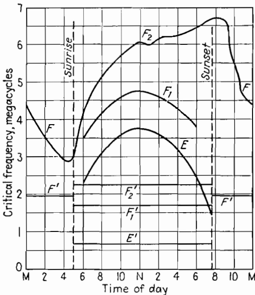
FIG. 168.—Method of predicting the performance of a 5,600-kc. frequency with time of day for a distance of 1,000 miles.
