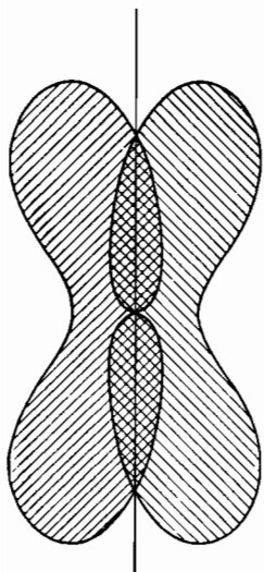
FIG. 123.—Horizontal-plane field pattern of the CAA-I.T.D. instrument-landing localizer.
