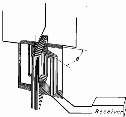
FIG. 150.—Mechanical structure of a goniometer used for direction finding and its method of connection. The coils connecting to the antennas are fixed and bear a 90-deg. relation to each other. The inner coil rotates.
