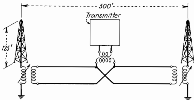
FIG. 25.—The TL radio-range antenna system.
