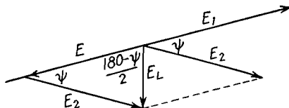
FIG. 64.—Voltage resulting from the vectorial addition of the voltages induced in the sides of the loop.
